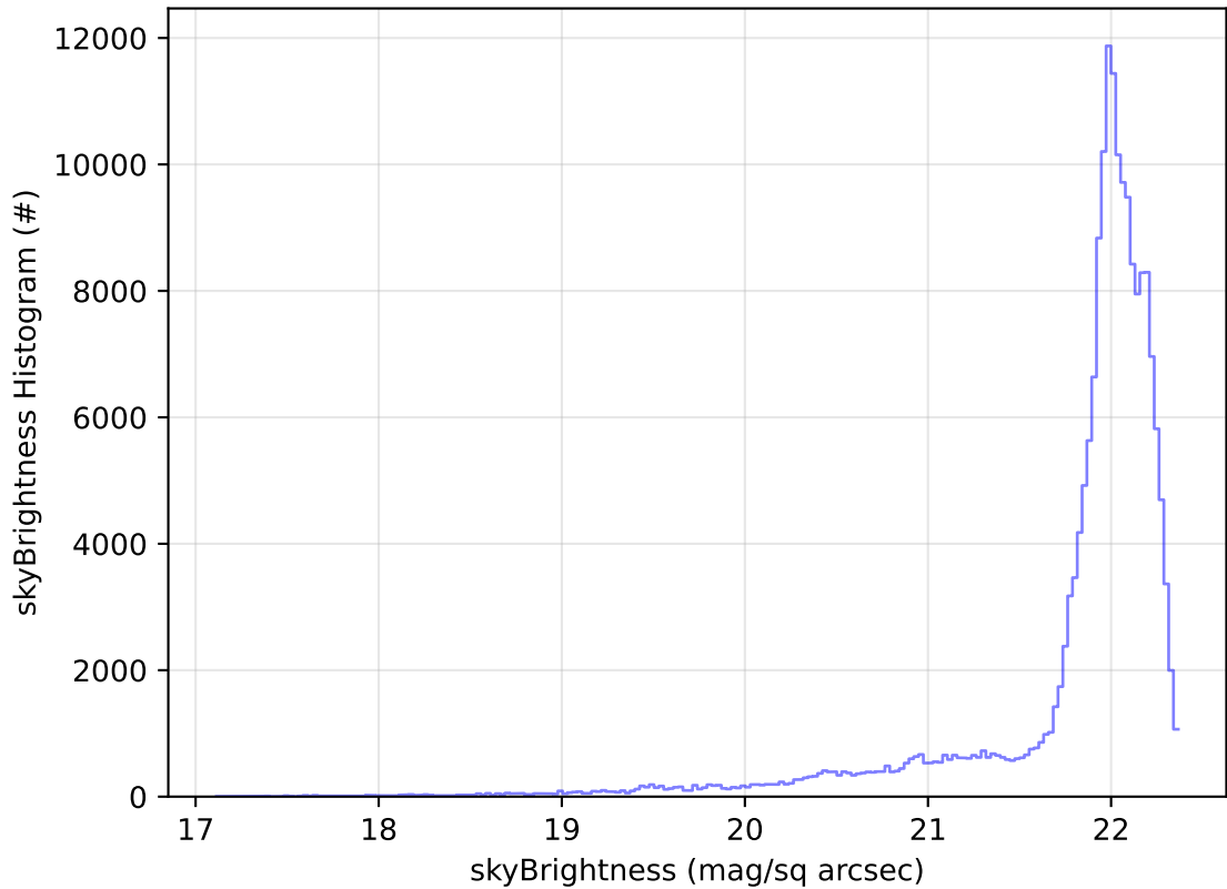
too_elab_2yr_r128_d3_ugrizy_v3.4_10yrs All sky g band: skyBrightness Histogram
