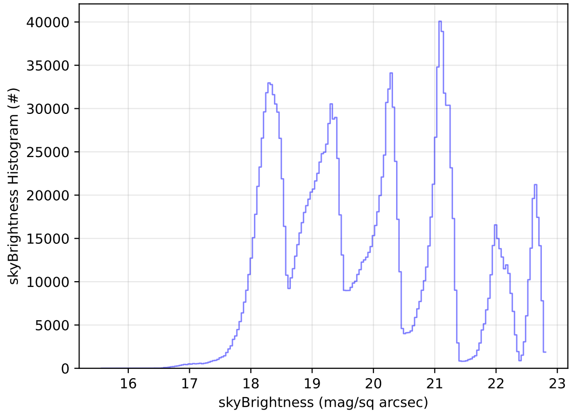
too_elab_2yr_r128_d3_ugrizy_v3.4_10yrs All sky all bands: skyBrightness Histogram
