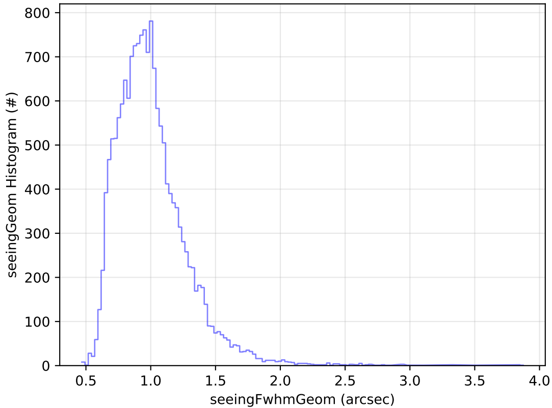
too_elab_2yr_r128_d3_ugrizy_v3.4_10yrs Yr 1 u band: seeingGeom Histogram
