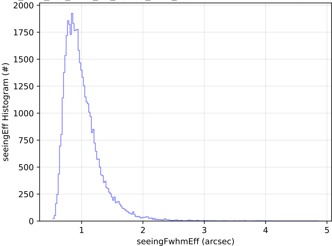
too_elab_2yr_r128_d3_ugrizy_v3.4_10yrs Yr 1 z band: seeingEff Histogram
