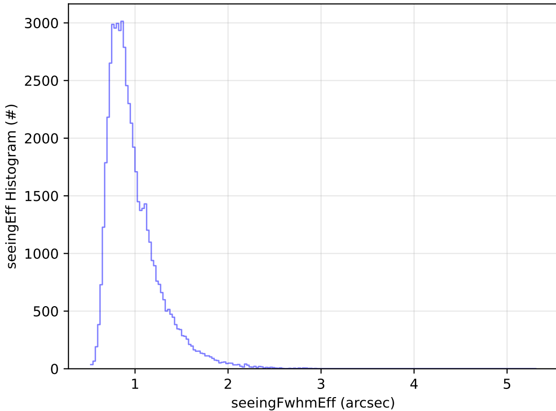
too_elab_2yr_r128_d3_ugrizy_v3.4_10yrs Yr 1 i band: seeingEff Histogram
