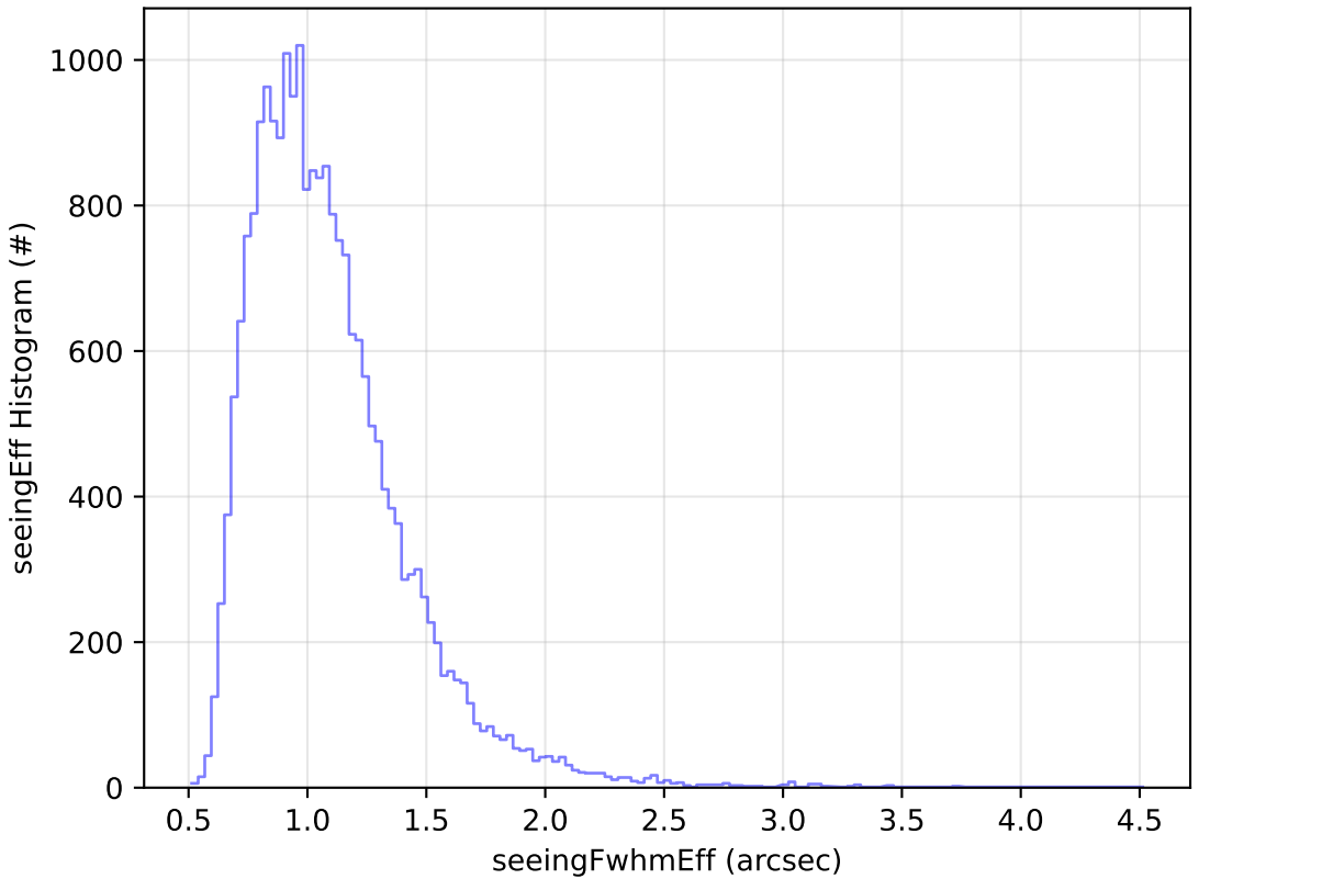
too_elab_2yr_r128_d3_ugrizy_v3.4_10yrs Yr 1 g band: seeingEff Histogram
