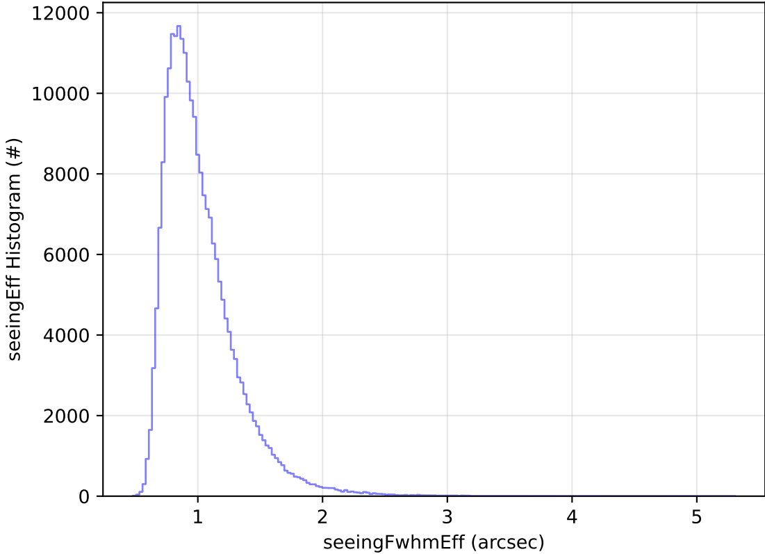
too_elab_2yr_r128_d3_ugrizy_v3.4_10yrs Yr 1 all bands: seeingEff Histogram
