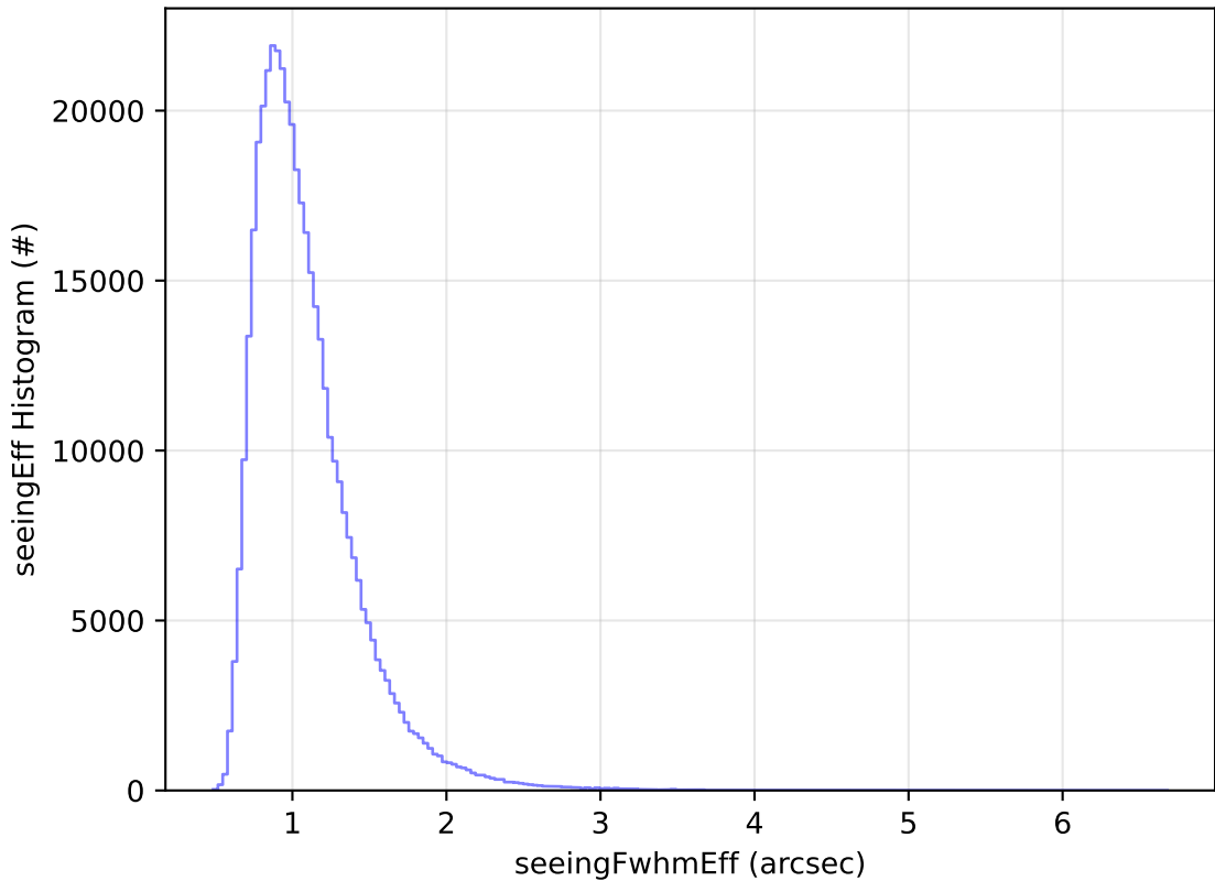
too_elab_2yr_r128_d3_ugrizy_v3.4_10yrs WFD z band: seeingEff Histogram
