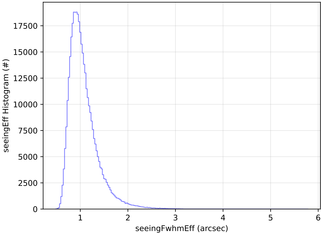
too_elab_2yr_r128_d3_ugrizy_v3.4_10yrs WFD y band: seeingEff Histogram
