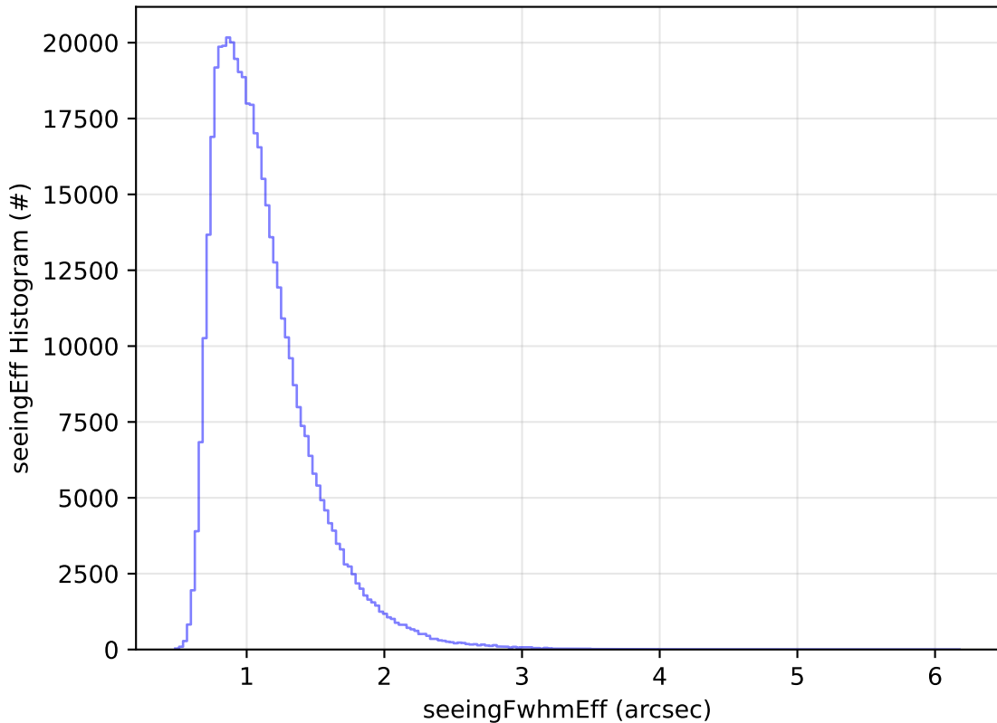
too_elab_2yr_r128_d3_ugrizy_v3.4_10yrs WFD r band: seeingEff Histogram
