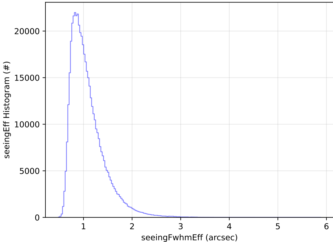
too_elab_2yr_r128_d3_ugrizy_v3.4_10yrs WFD i band: seeingEff Histogram
