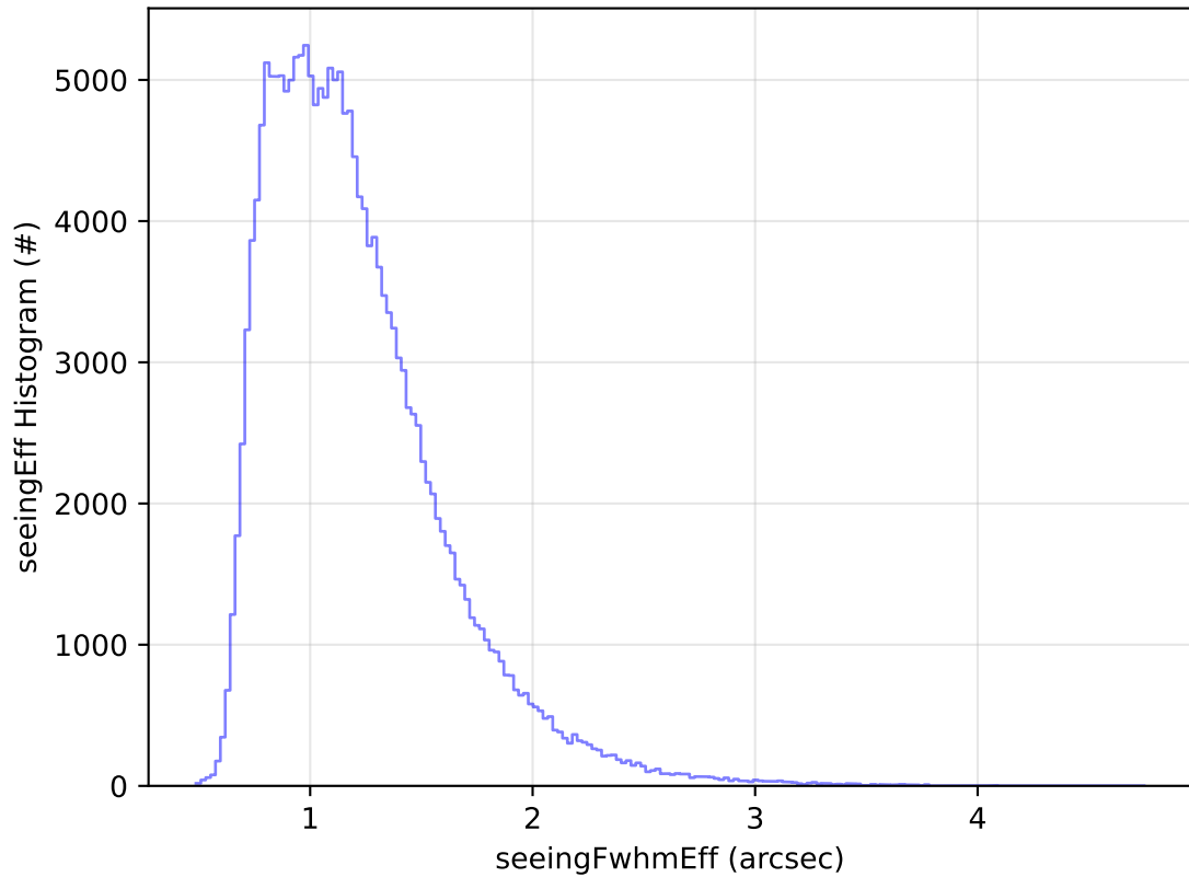
too_elab_2yr_r128_d3_ugrizy_v3.4_10yrs WFD g band: seeingEff Histogram
