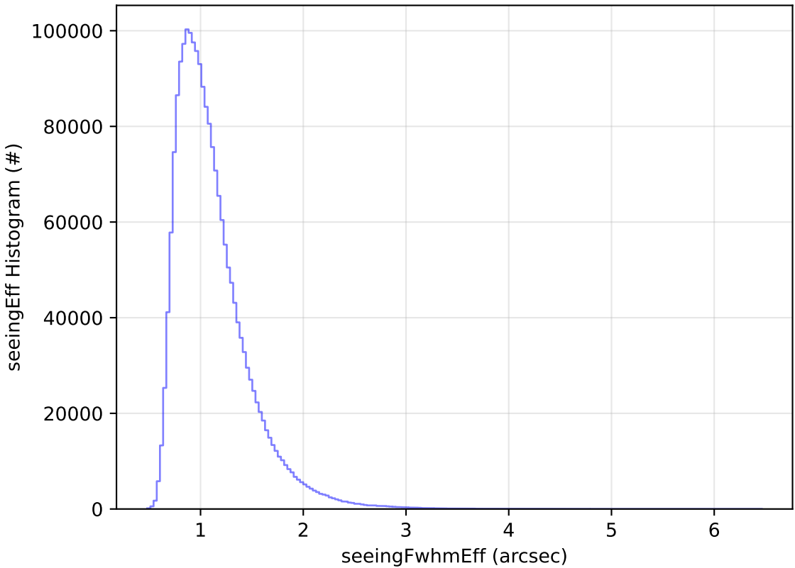
too_elab_2yr_r128_d3_ugrizy_v3.4_10yrs WFD all bands: seeingEff Histogram
