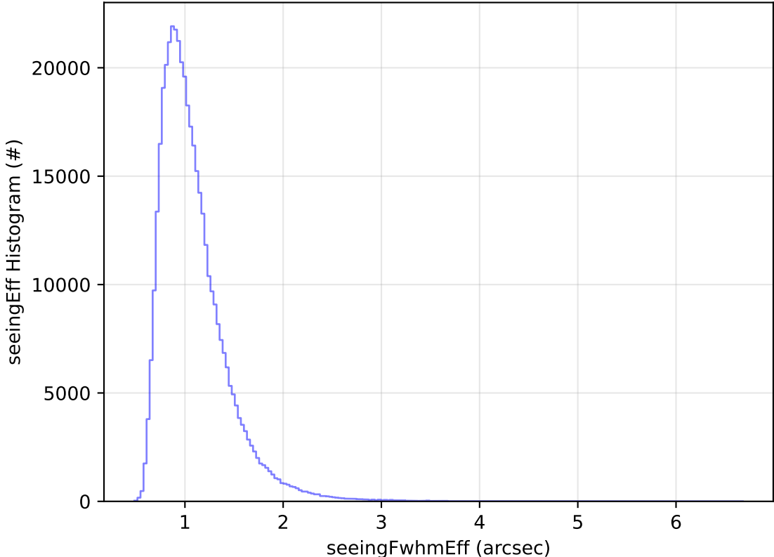
too_elab_2yr_r128_d3_ugrizy_v3.4_10yrs All sky z band: seeingEff Histogram
