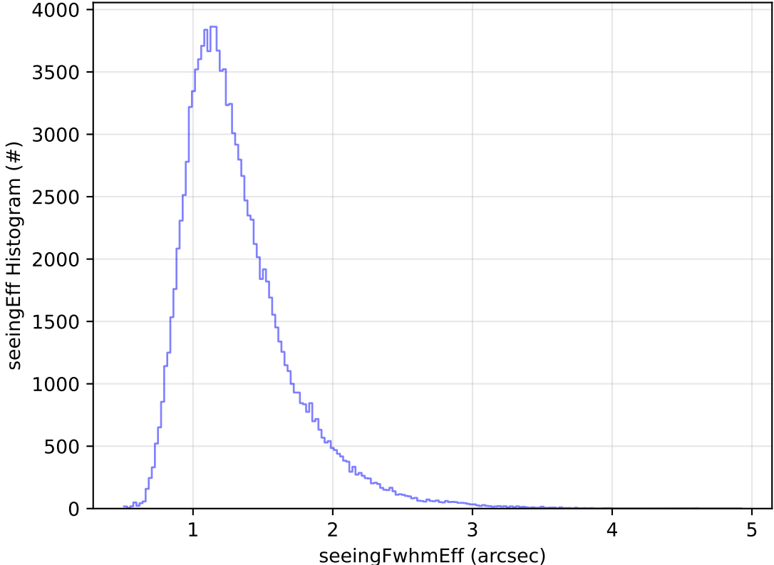
too_elab_2yr_r128_d3_ugrizy_v3.4_10yrs All sky u band: seeingEff Histogram
