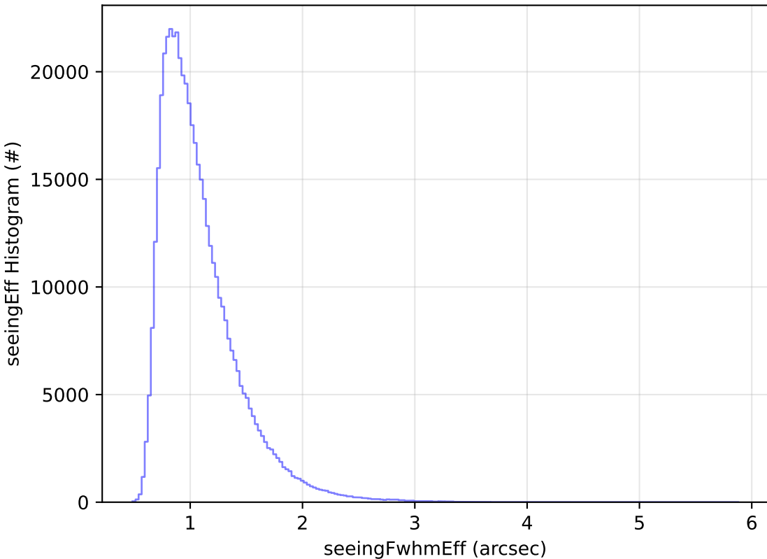
too_elab_2yr_r128_d3_ugrizy_v3.4_10yrs All sky i band: seeingEff Histogram
