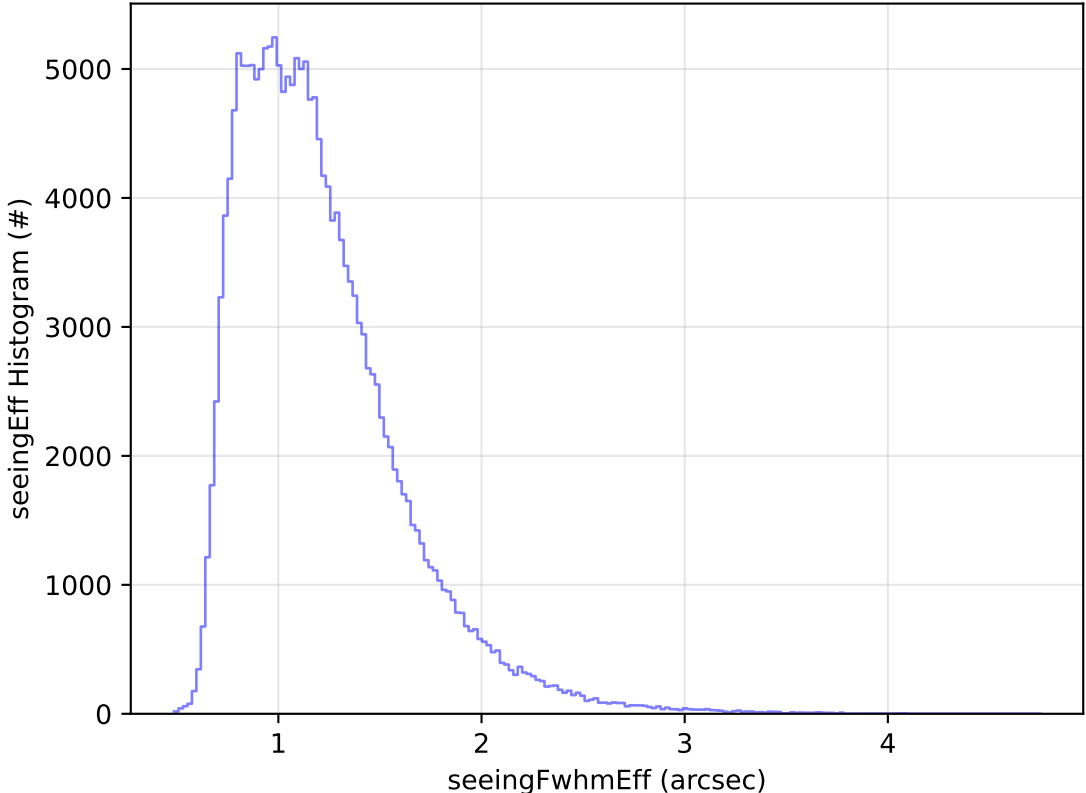
too_elab_2yr_r128_d3_ugrizy_v3.4_10yrs All sky g band: seeingEff Histogram
