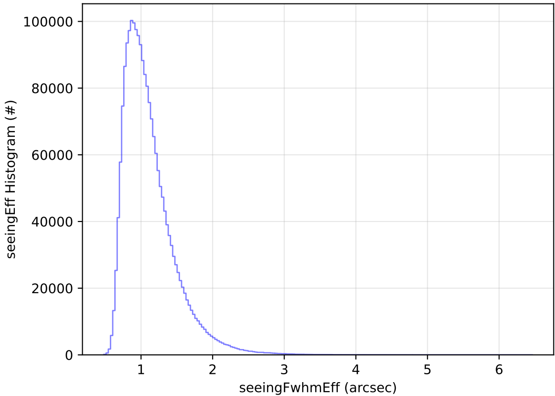
too_elab_2yr_r128_d3_ugrizy_v3.4_10yrs All sky all bands: seeingEff Histogram
