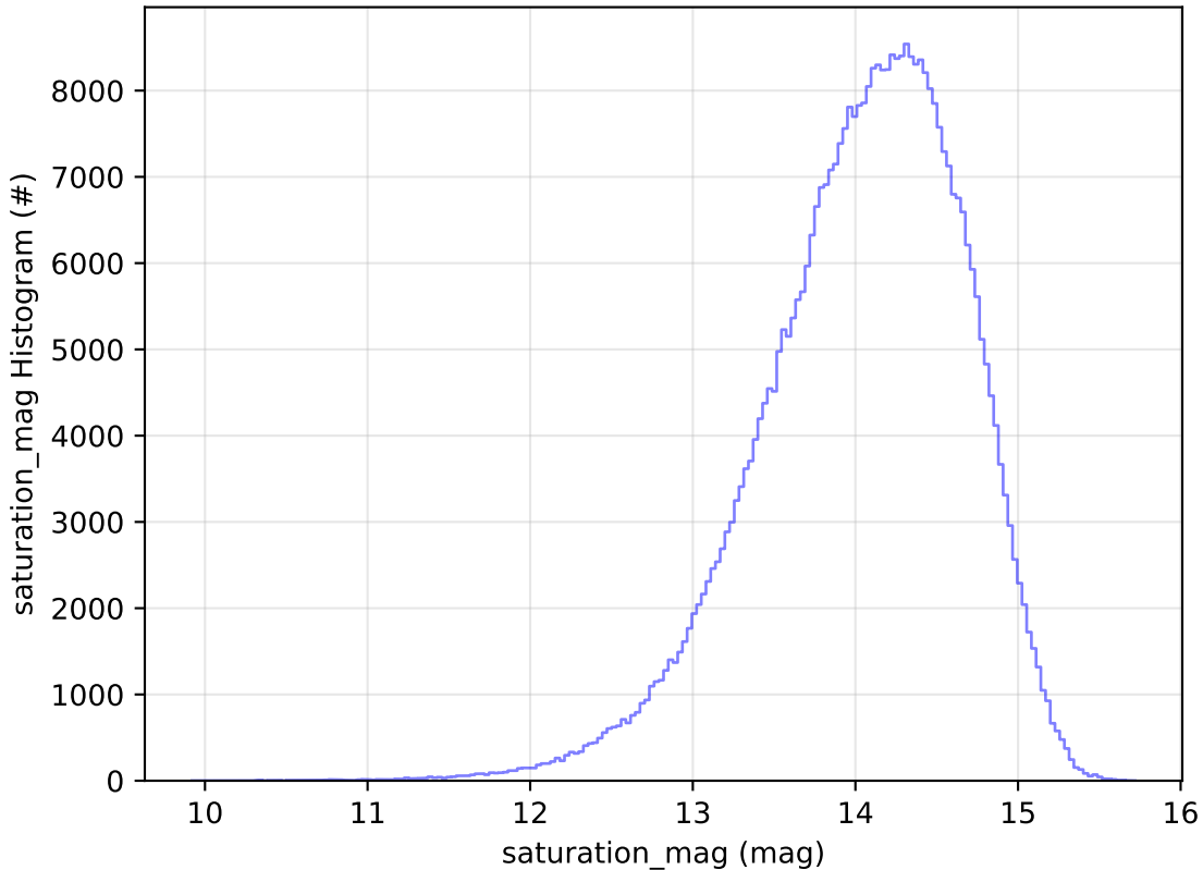
too_elab_2yr_r128_d3_ugrizy_v3.4_10yrs WFD z band: saturation_mag Histogram
