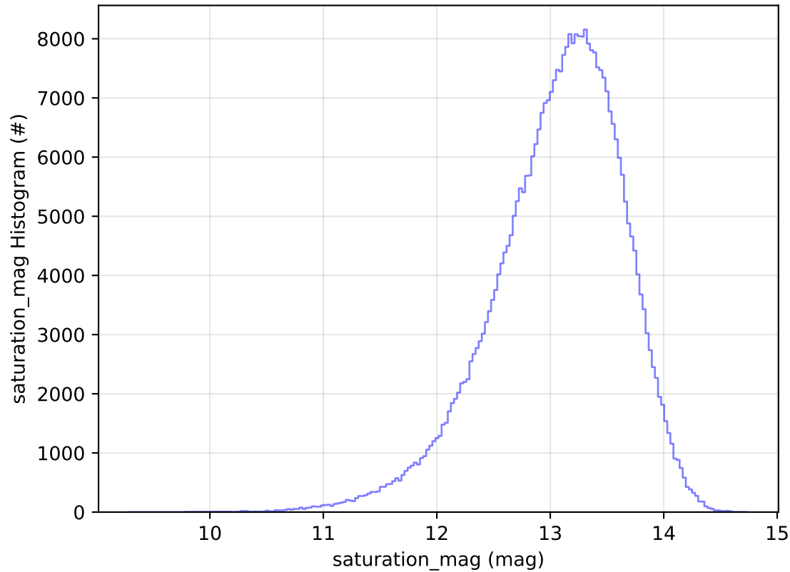
too_elab_2yr_r128_d3_ugrizy_v3.4_10yrs WFD y band: saturation_mag Histogram
