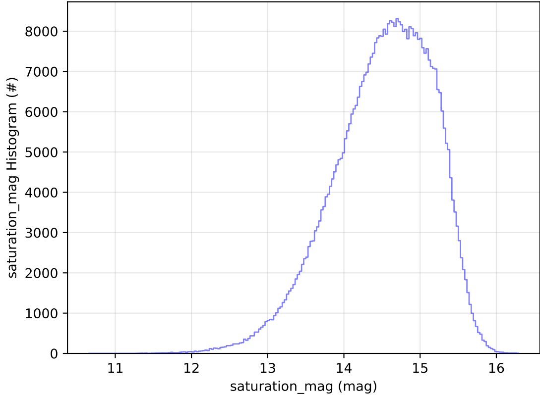
too_elab_2yr_r128_d3_ugrizy_v3.4_10yrs WFD r band: saturation_mag Histogram
