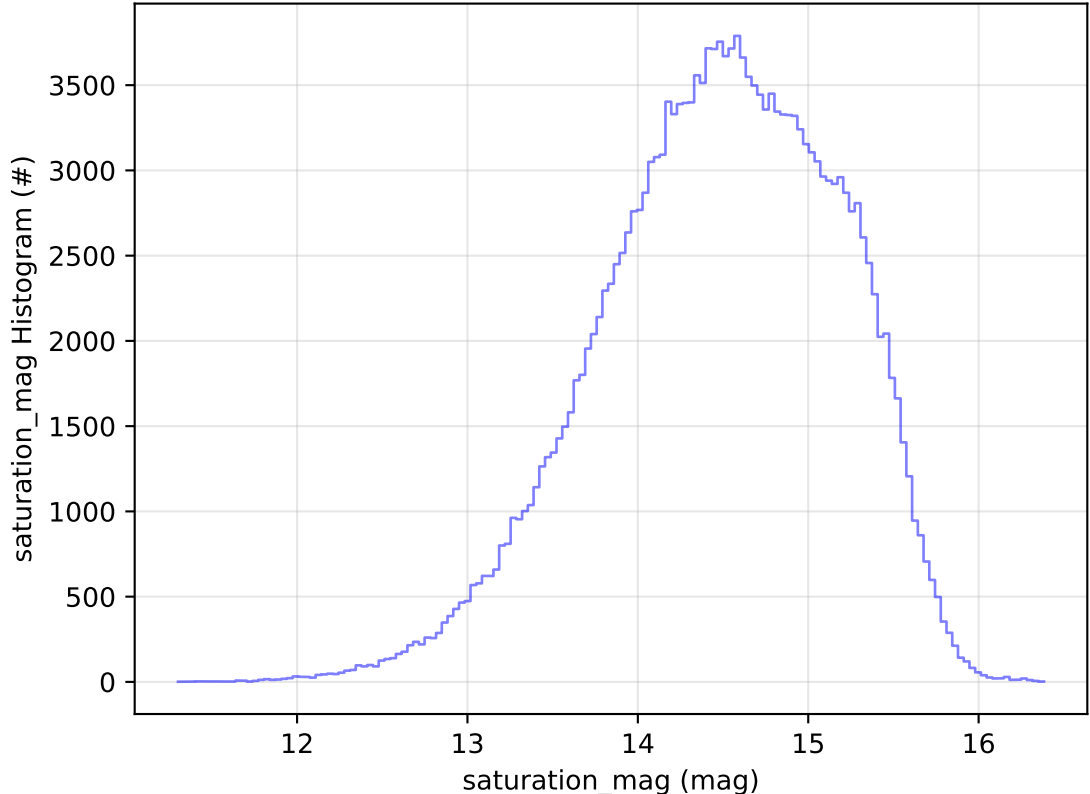
too_elab_2yr_r128_d3_ugrizy_v3.4_10yrs WFD g band: saturation_mag Histogram
