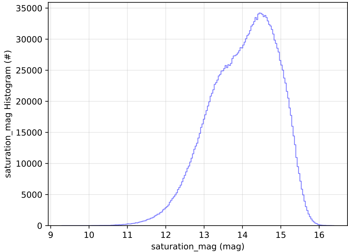
too_elab_2yr_r128_d3_ugrizy_v3.4_10yrs WFD all bands: saturation_mag Histogram
