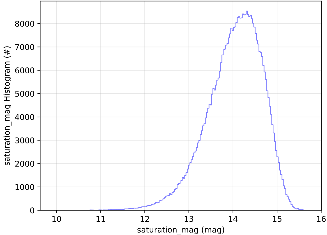
too_elab_2yr_r128_d3_ugrizy_v3.4_10yrs All sky z band: saturation_mag Histogram
