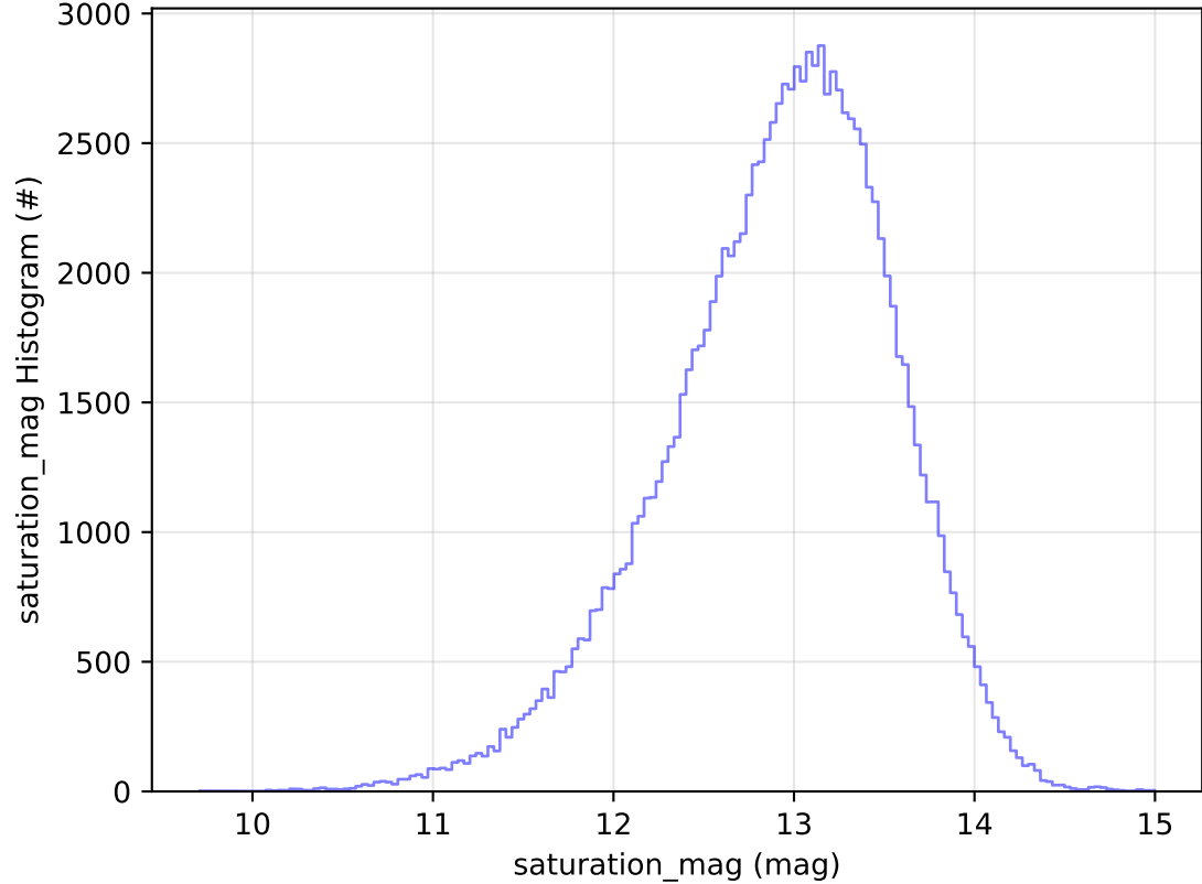
too_elab_2yr_r128_d3_ugrizy_v3.4_10yrs All sky u band: saturation_mag Histogram
