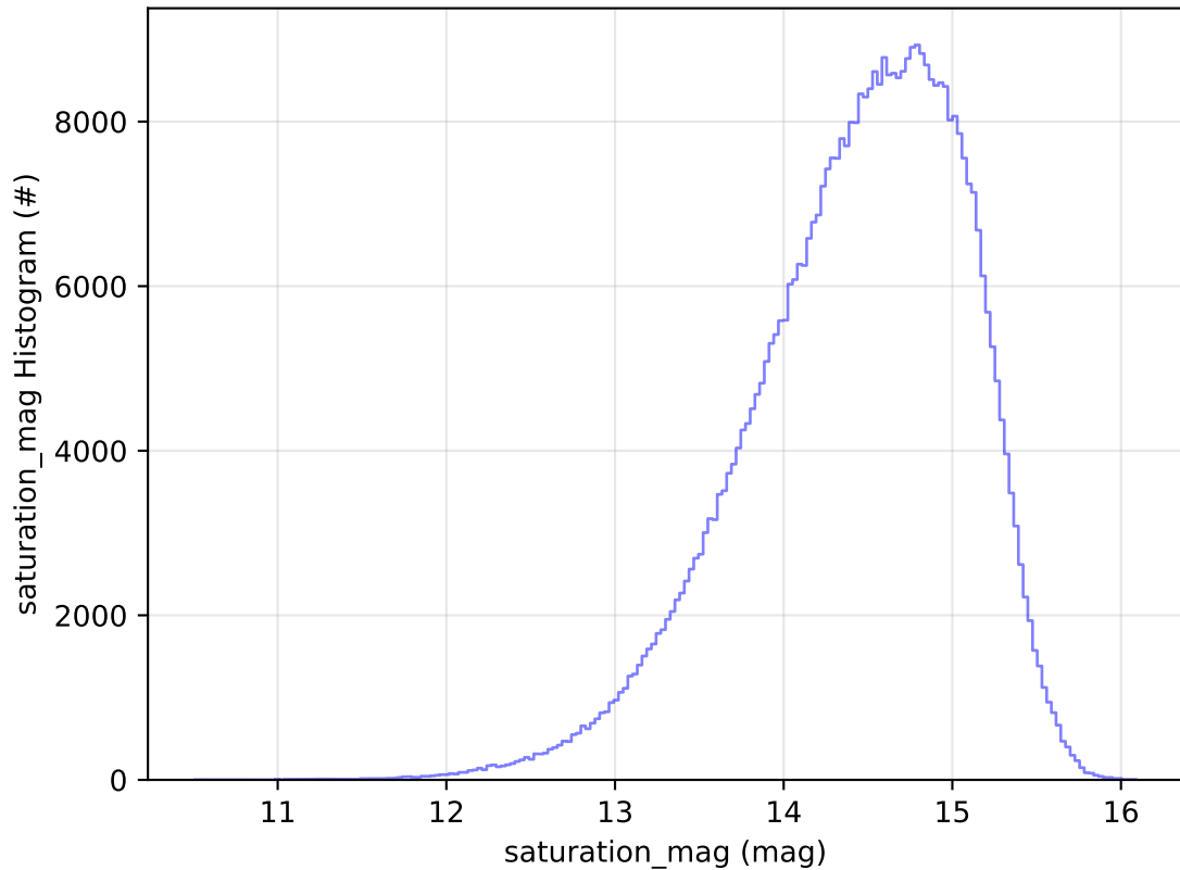
too_elab_2yr_r128_d3_ugrizy_v3.4_10yrs All sky i band: saturation_mag Histogram
