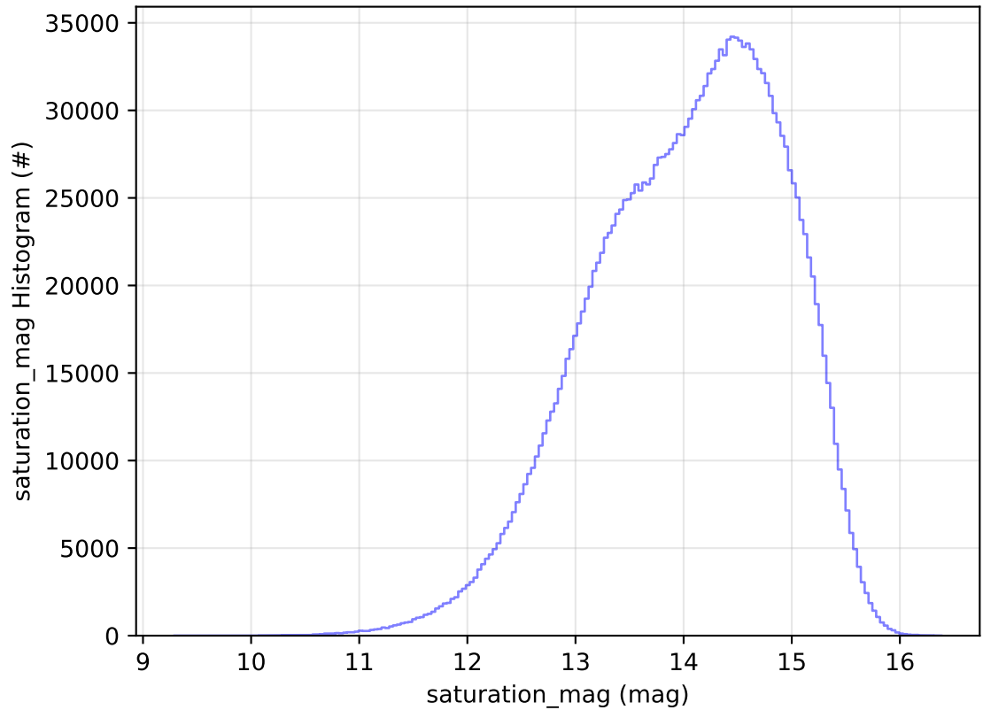
too_elab_2yr_r128_d3_ugrizy_v3.4_10yrs All sky all bands: saturation_mag Histogram
