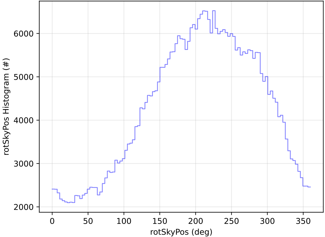
too_elab_2yr_r128_d3_ugrizy_v3.4_10yrs WFD z band: rotSkyPos Histogram
