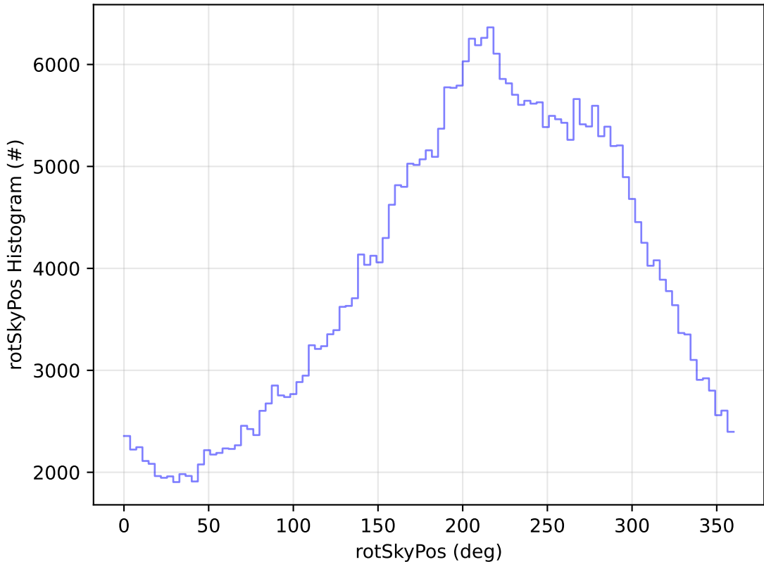
too_elab_2yr_r128_d3_ugrizy_v3.4_10yrs WFD y band: rotSkyPos Histogram
