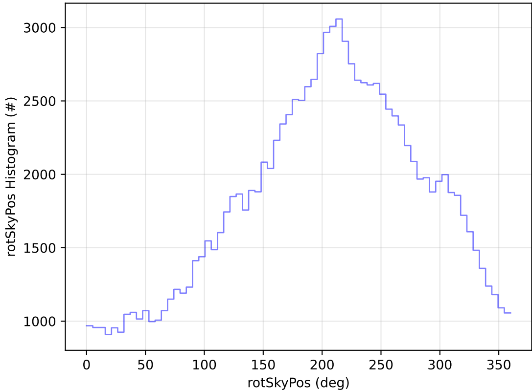
too_elab_2yr_r128_d3_ugrizy_v3.4_10yrs WFD u band: rotSkyPos Histogram
