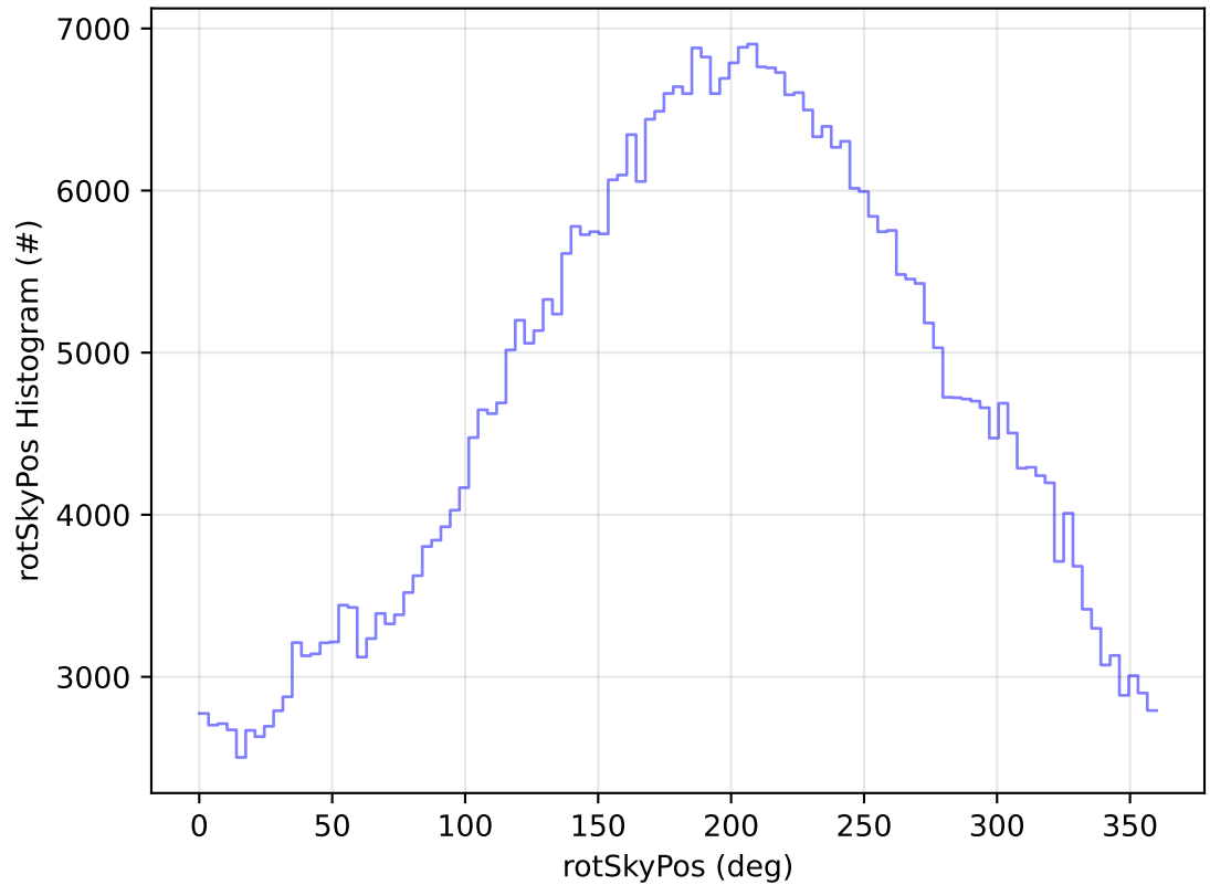
too_elab_2yr_r128_d3_ugrizy_v3.4_10yrs WFD r band: rotSkyPos Histogram
