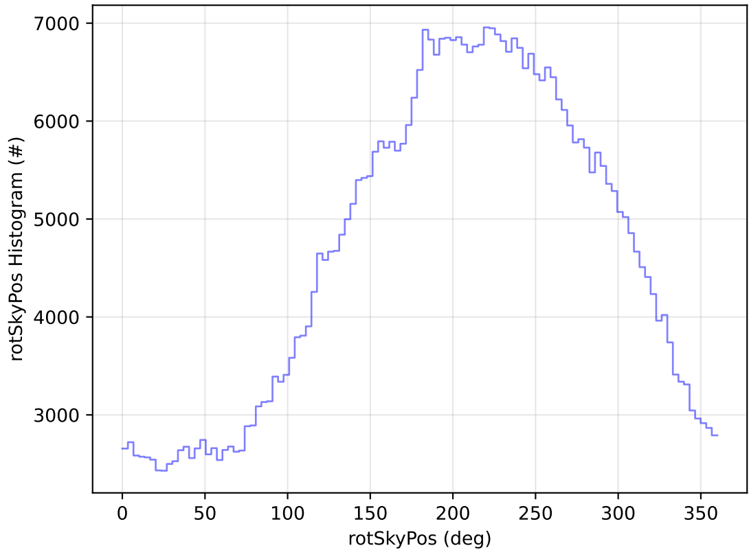
too_elab_2yr_r128_d3_ugrizy_v3.4_10yrs WFD i band: rotSkyPos Histogram
