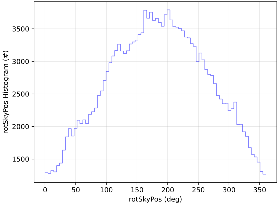
too_elab_2yr_r128_d3_ugrizy_v3.4_10yrs WFD g band: rotSkyPos Histogram
