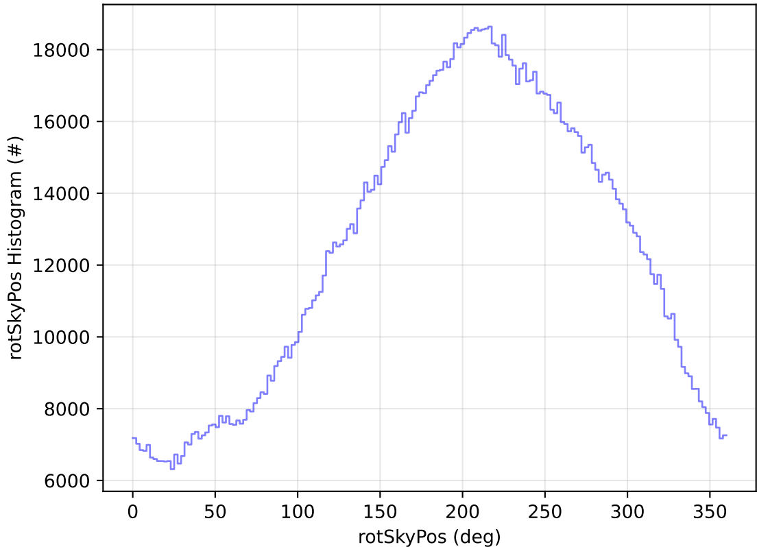
too_elab_2yr_r128_d3_ugrizy_v3.4_10yrs WFD all bands: rotSkyPos Histogram
