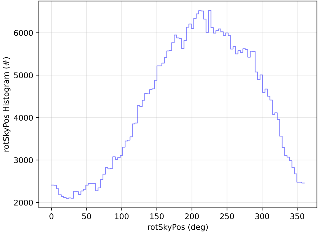
too_elab_2yr_r128_d3_ugrizy_v3.4_10yrs All sky z band: rotSkyPos Histogram
