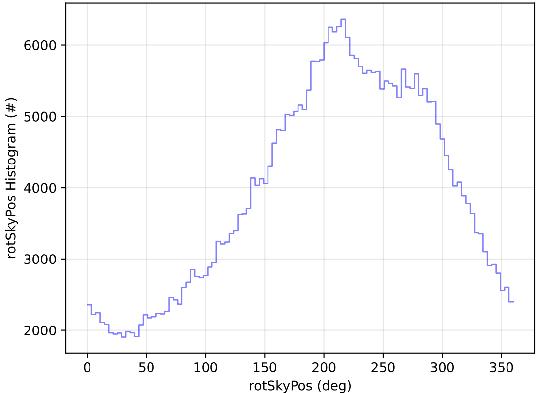
too_elab_2yr_r128_d3_ugrizy_v3.4_10yrs All sky y band: rotSkyPos Histogram
