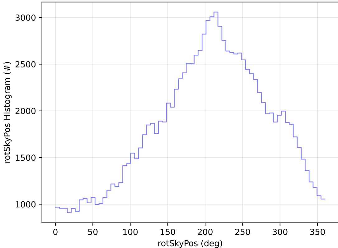
too_elab_2yr_r128_d3_ugrizy_v3.4_10yrs All sky u band: rotSkyPos Histogram
