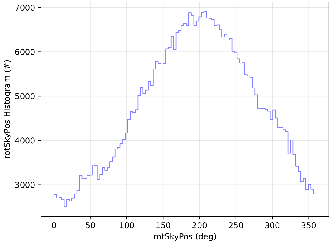
too_elab_2yr_r128_d3_ugrizy_v3.4_10yrs All sky r band: rotSkyPos Histogram
