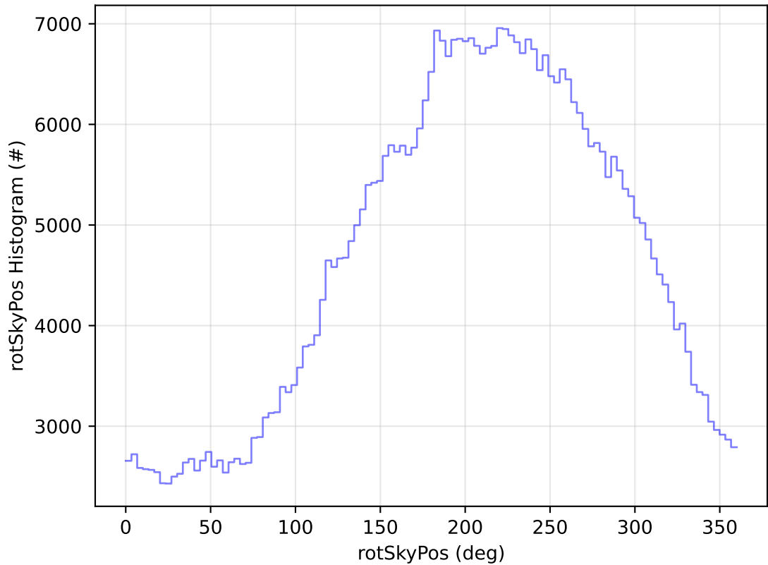
too_elab_2yr_r128_d3_ugrizy_v3.4_10yrs All sky i band: rotSkyPos Histogram
