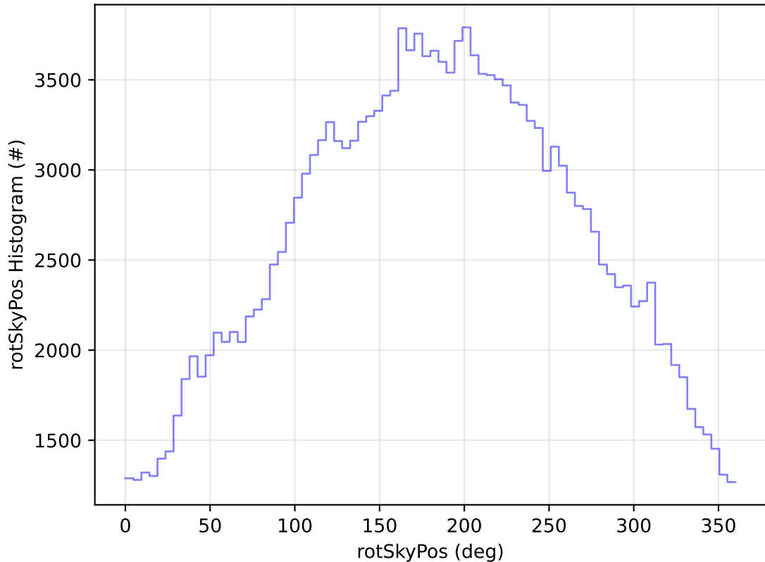
too_elab_2yr_r128_d3_ugrizy_v3.4_10yrs All sky g band: rotSkyPos Histogram
