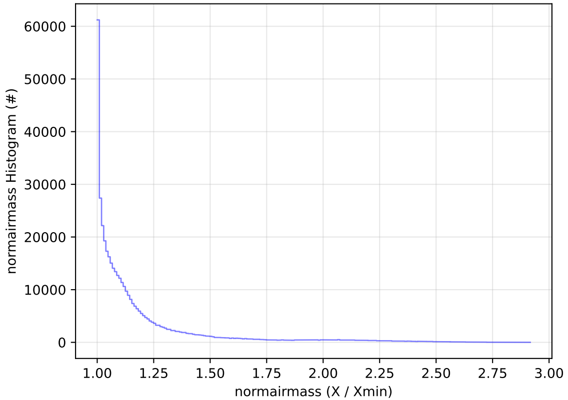
too_elab_2yr_r128_d3_ugrizy_v3.4_10yrs WFD z band: normairmass Histogram
