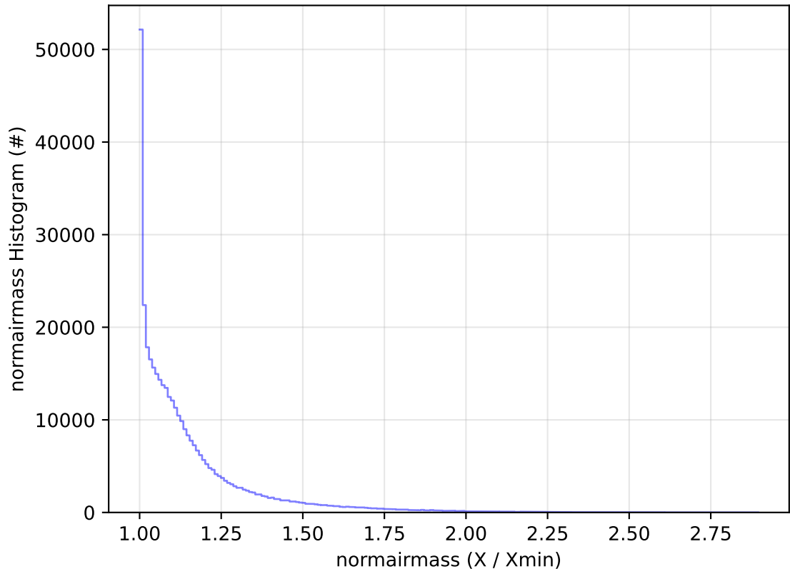
too_elab_2yr_r128_d3_ugrizy_v3.4_10yrs WFD y band: normairmass Histogram
