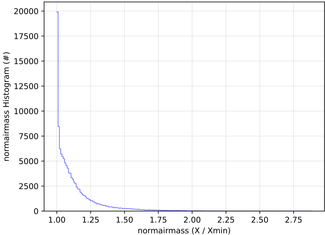
too_elab_2yr_r128_d3_ugrizy_v3.4_10yrs WFD u band: normairmass Histogram
