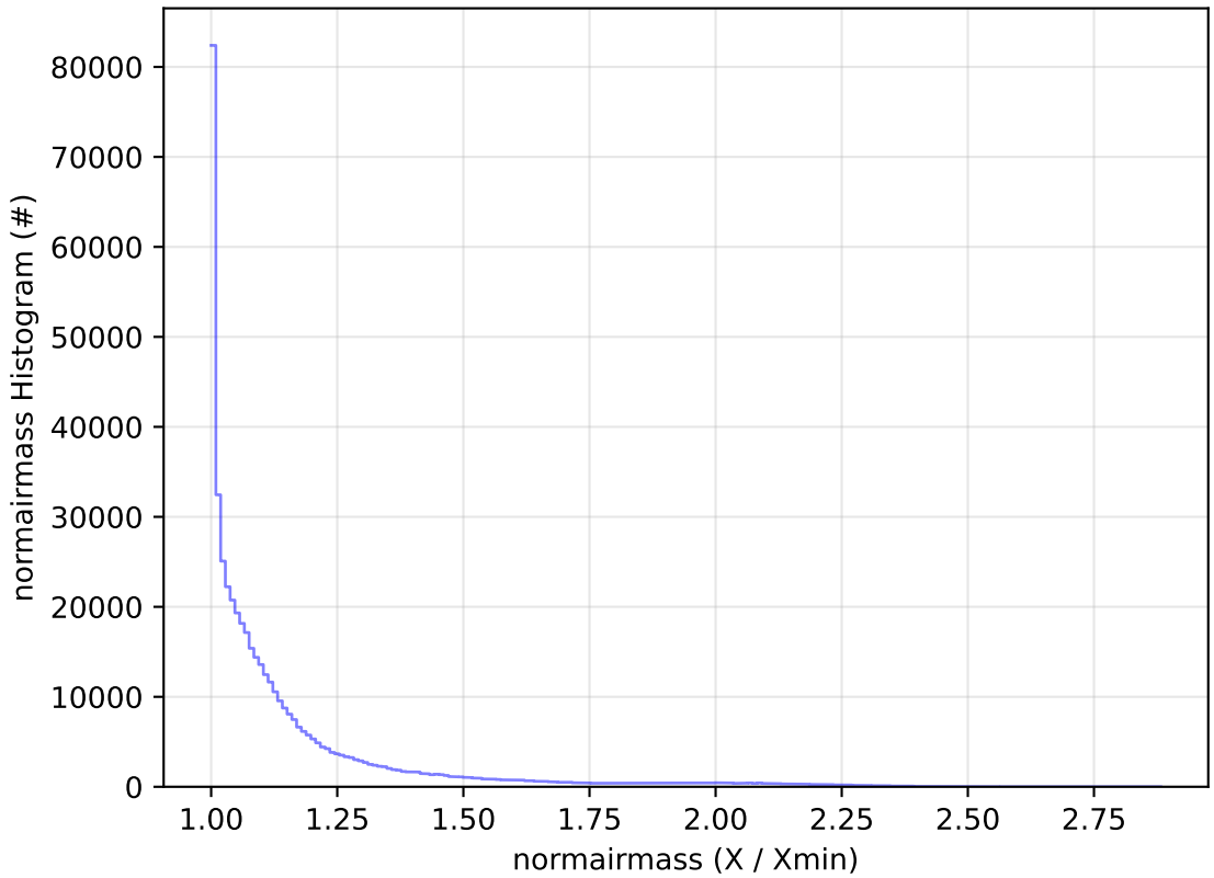
too_elab_2yr_r128_d3_ugrizy_v3.4_10yrs WFD r band: normairmass Histogram
