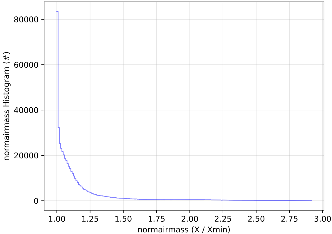
too_elab_2yr_r128_d3_ugrizy_v3.4_10yrs WFD i band: normairmass Histogram
