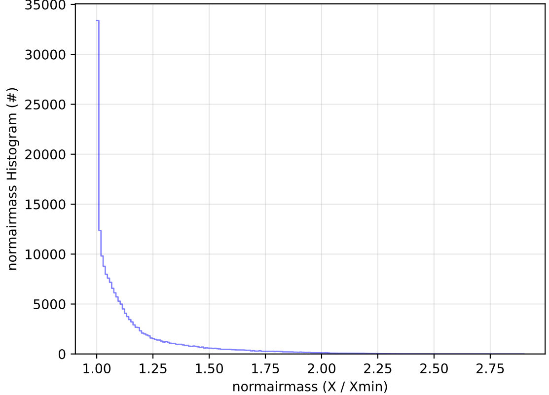
too_elab_2yr_r128_d3_ugrizy_v3.4_10yrs WFD g band: normairmass Histogram
