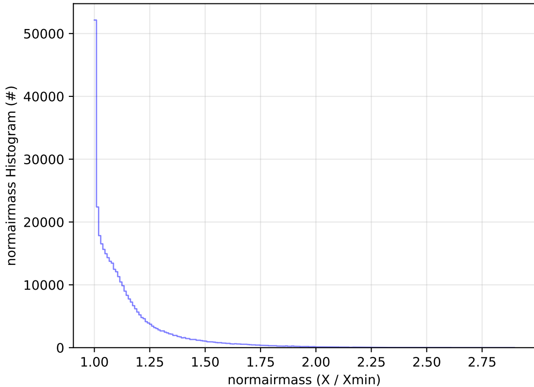
too_elab_2yr_r128_d3_ugrizy_v3.4_10yrs All sky y band: normairmass Histogram
