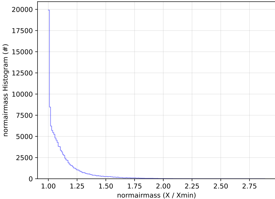
too_elab_2yr_r128_d3_ugrizy_v3.4_10yrs All sky u band: normairmass Histogram
