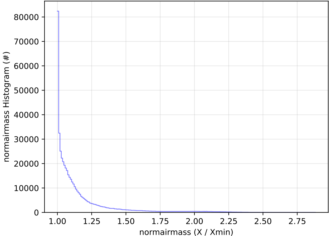
too_elab_2yr_r128_d3_ugrizy_v3.4_10yrs All sky r band: normairmass Histogram
