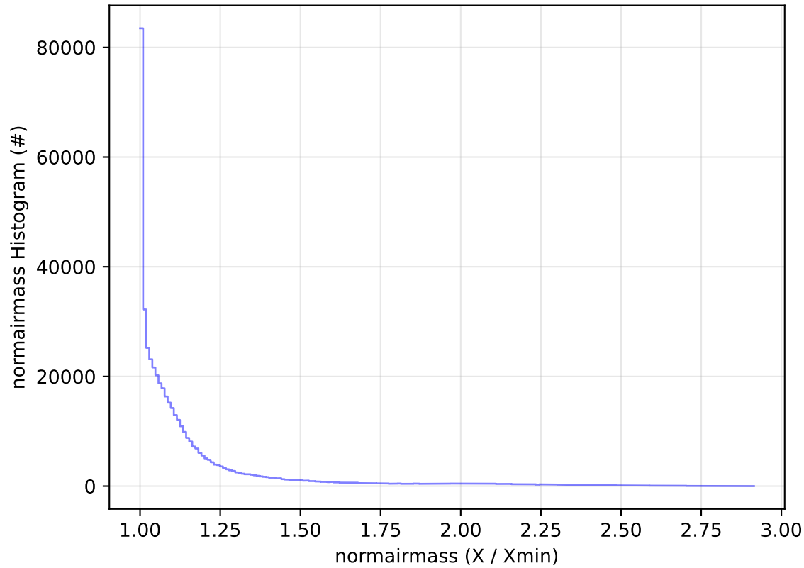
too_elab_2yr_r128_d3_ugrizy_v3.4_10yrs All sky i band: normairmass Histogram
